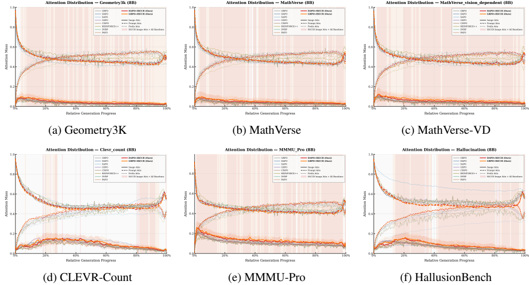
Figure 8: 8B RLVR attention dynamics. HiCCR sustains higher image attention across benchmarks, while GRPO, DAPO, and related RLVR baselines exhibit progressive visual-attention drift.
