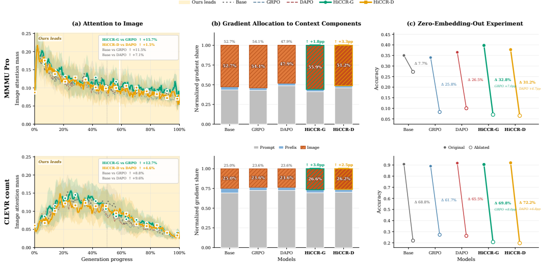
Figure 1: RLVR fine-tuning weakens visual grounding in MLLMs, and HiCCR mitigates it.
