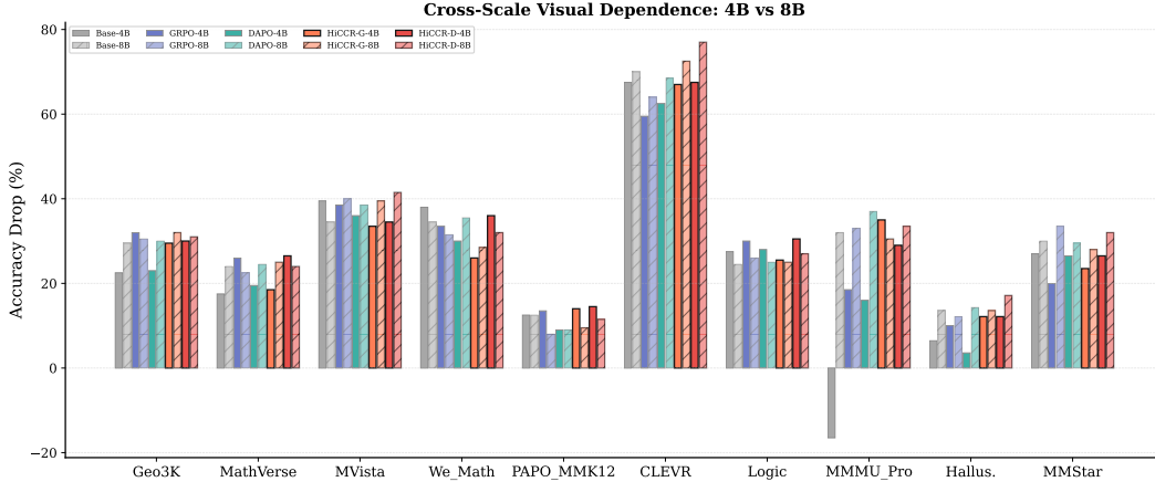
Figure 7: Cross-Scale Counterfactual Visual Ablation. We report the accuracy drop (%) when visual embeddings are zeroed out during inference. A larger drop indicates stronger functional dependence on visual inputs. Across both 4B (solid) and 8B (hatched) scales, HiCCR variants consistently exhibit the most severe performance degradation upon visual corruption, confirming that our method substantially enforces stronger visual functional dependence.
