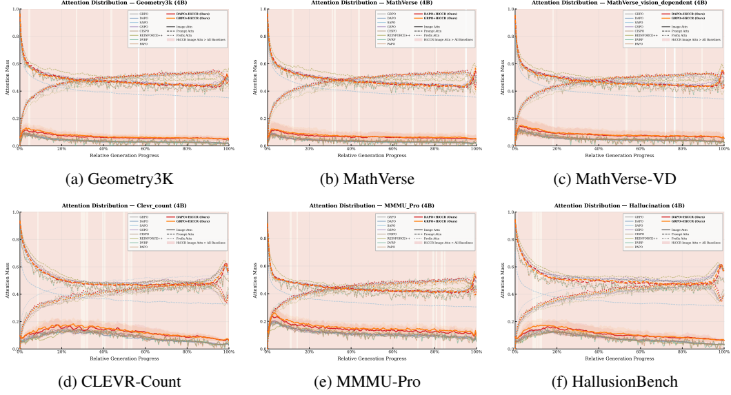
Figure 9: 4B RLVR attention dynamics. Attention drift becomes stronger at the smaller scale, but HiCCR still preserves a stable visual attention plateau beyond all RLVR baselines.
