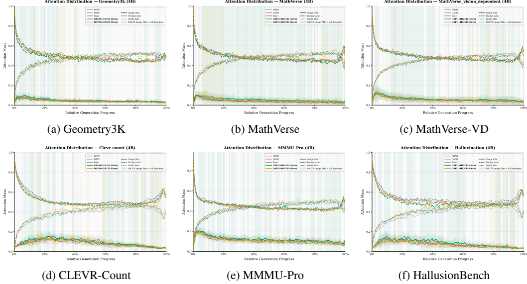
Figure 11: 4B base-model attention comparison. The 4B base model suffers stronger visual-attention collapse, which GRPO and DAPO further reinforce while HiCCR effectively restores sustained image attention.
