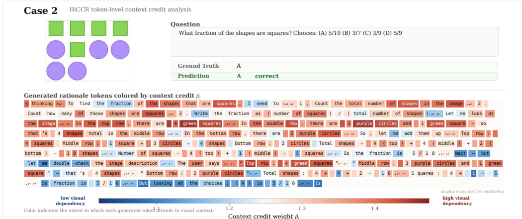
Figure 13: Case 2: fraction of shapes (ViRL39K training rollout) . Shape- and color-descriptive tokens (“green squares”, “purple circles”, row-wise counts) carry the largest weights, while arithmetic tokens (“5/10”, “Is”) fall into the low-dependency band, indicating that credit follows perceptual evidence rather than downstream calculation.
