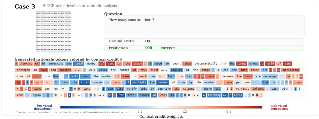
Figure 14: Case 3: counting 10×10 cans (ViRL39K training rollout) . HiCCR assigns high credit to structural-perception tokens (“grid”, “rows”, “columns”, “10 horizontal rows”), while the multiplicative closure (“10 × 10 = 100”) and the answer tag receive near-unity weight, a clean separation between “looking” and “computing”.
