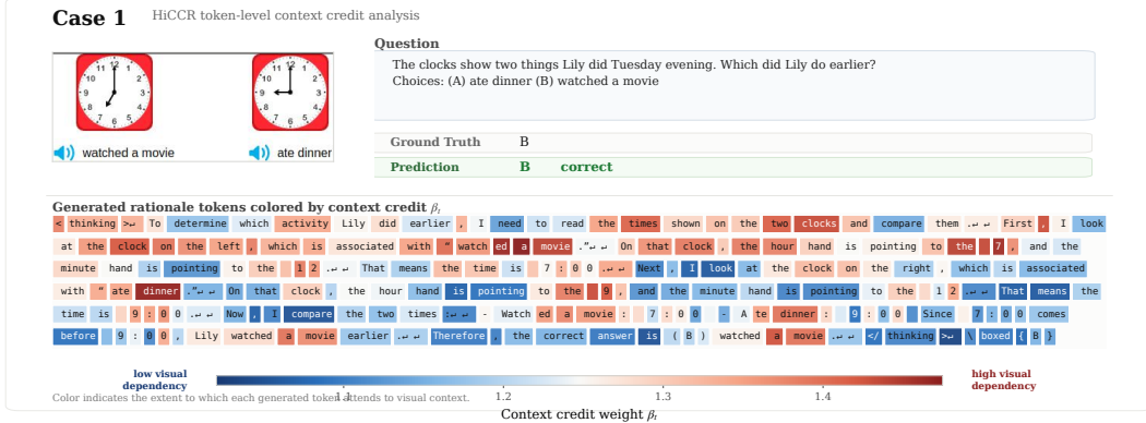
Figure 12: Case 1: clock reading (ViRL39K training rollout) . Tokens referring to clock positions (“7”, “9”, “pointing”, “clock”, “movie/dinner”) receive the highest credit, while temporal comparison tokens (“before”, “Since”, “Therefore”) drop to near-baseline weight, showing that HiCCR amplifies visually grounded time reading rather than purely textual reasoning.
