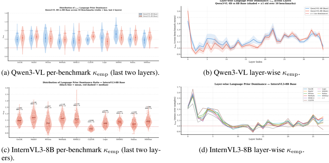
Figure 6: Empirical support for the absolute-scale component of language-prior dominance. Across the evaluated benchmarks and model families, \kappa_{\text{emp}} is consistently above one in the measured layers, suggesting that non-visual context often carries larger downstream-projected activation magnitude than visual context.
