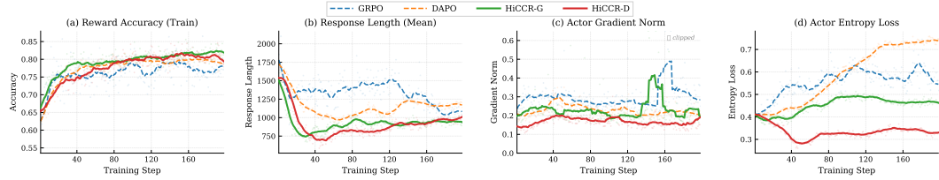
Figure 3: Training dynamics on Qwen3-VL-4B. (a) Reward accuracy. (b) Mean response length. (c) Actor gradient norm. (d) Policy entropy. Faint dots show per-step values; solid/dashed lines are smoothed averages. HiCCR converges to higher accuracy with shorter responses, stable gradients, and lower entropy, indicating efficient and confident visual reasoning.
