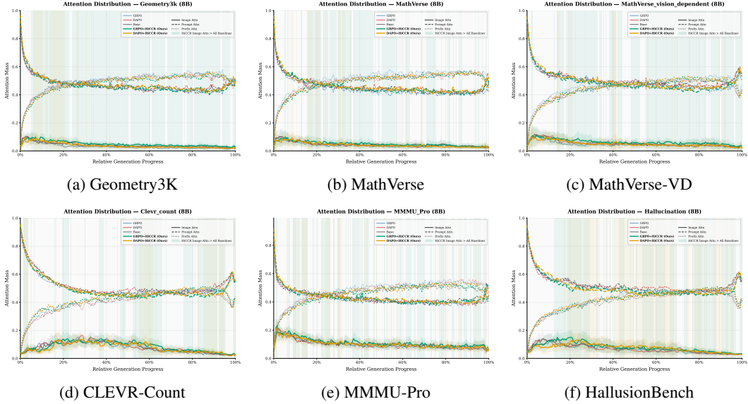
Figure 10: 8B base-model attention comparison. The pretrained base model already shows visual-attention decay, GRPO and DAPO amplify it, and HiCCR reverses the trend.
