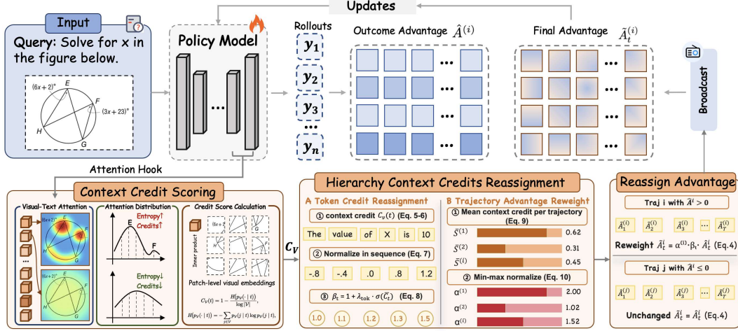
Figure 2: Overview of HiCCR. An attention hook on the policy model produces a per-token context credit C_V(t) from intra-visual attention entropy. Token- and trajectory-level weights \beta_t, \alpha^{(i)} are derived from C_V and reassign the outcome advantage as \tilde{A}_t^{(i)} = \alpha^{(i)} \beta_t \hat{A}^{(i)} . The reassignment is applied only to positive-advantage trajectories.
