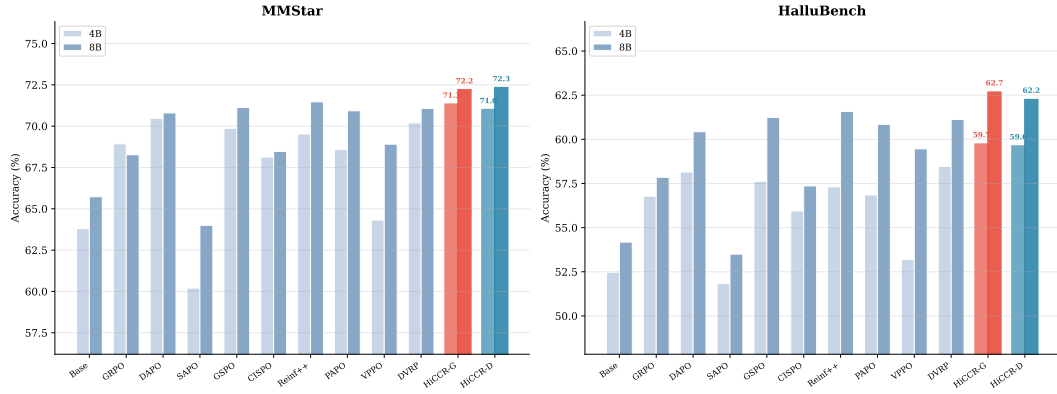
Figure 5: Performance on MMStar and HalluBench. Grouped bars compare all methods on Qwen3-VL-4B and 8B backbones. HiCCR variants (red/blue) consistently achieve the highest accuracy on both benchmarks, indicating improved visual perception and reduced hallucination.
