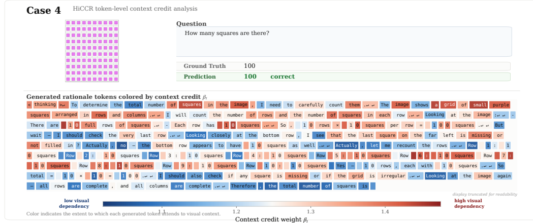
Figure 15: Case 4: counting 10 \times 10 squares with self-verification (ViRL39K training rollout). Even in a rollout containing a self-check sub-trajectory (“But wait – I should check the very last row”), HiCCR consistently upweights the row-wise enumeration tokens (Row 1–Row 10, “squares”), showing that the credit signal is robust to reasoning detours.
